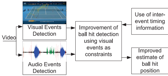
Figure 1: Overview of our approach to ball hit detection using high-level multi modal information. Visually detected ball-hits are used as a constraint on the position of audio-detected ball hits. Inter ball hit timing information is also used.
