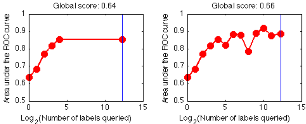
Figure 1: Examples of learning curves for 5 and 13 experimental points.
