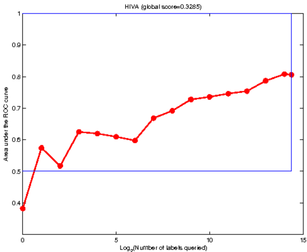
Baseline results on HIVA by Gavin Cawley.
