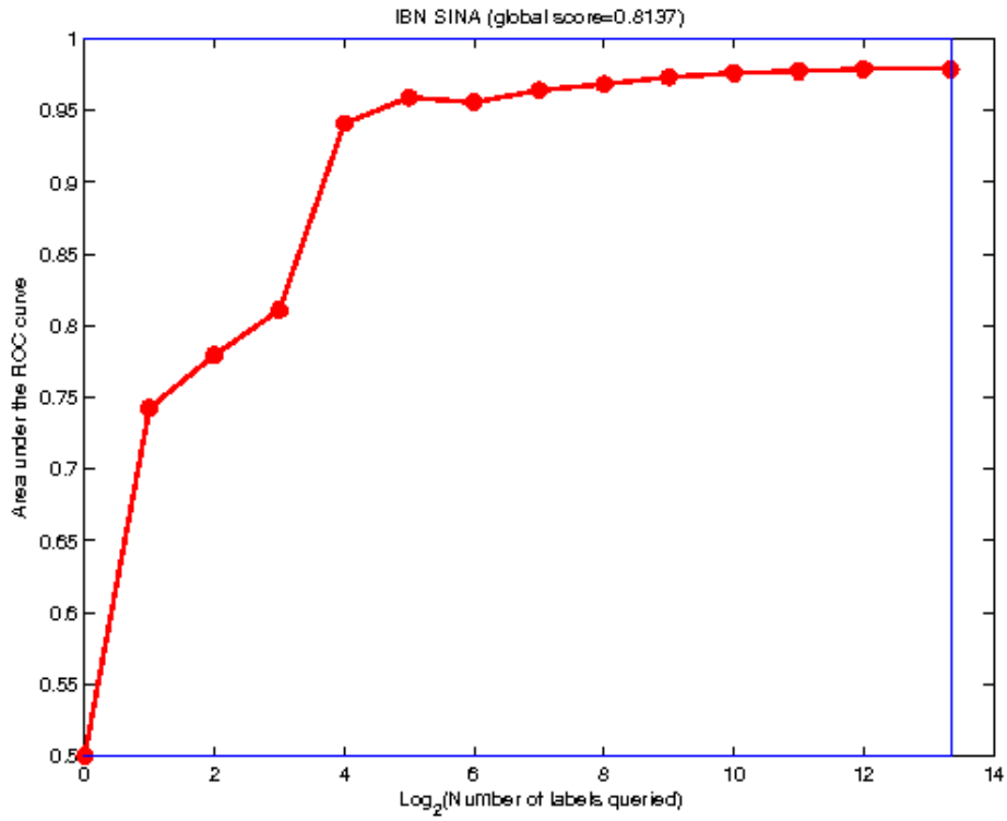
Reference results produced by Gavin Cawley on IBN_SINA.
