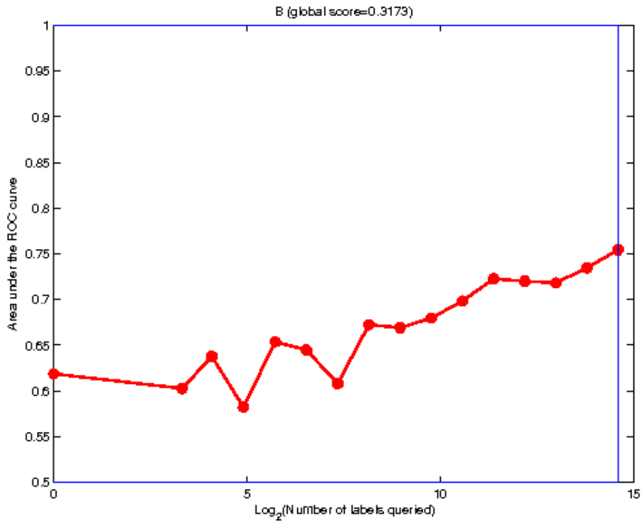
Results of Ideal Analytics, Intel, on the B dataset.
