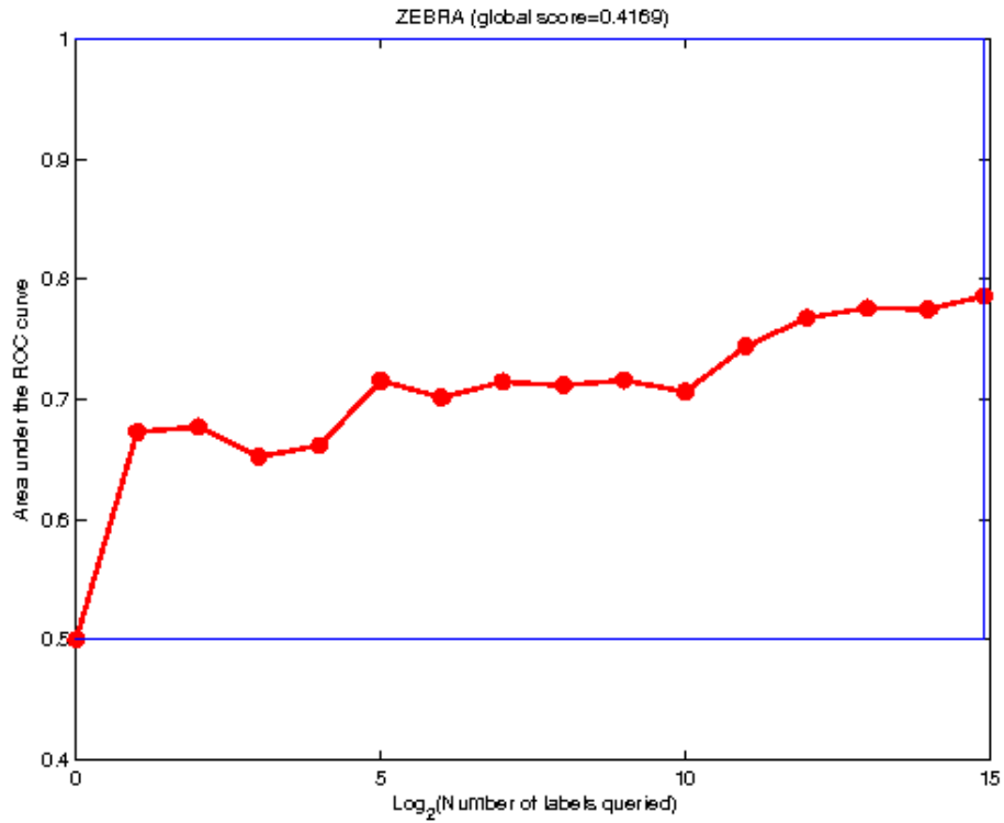
Reference result by Gavin Cawley on ZEBRA.
