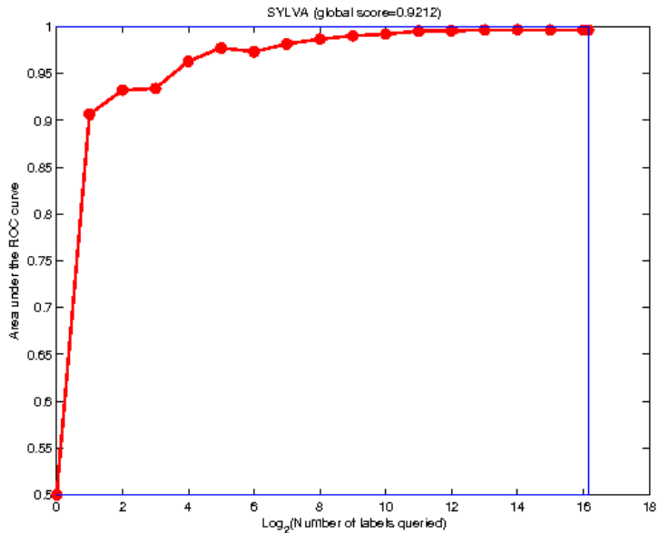
Baseline results obtained by Gavin Cawley on SYLVA.
