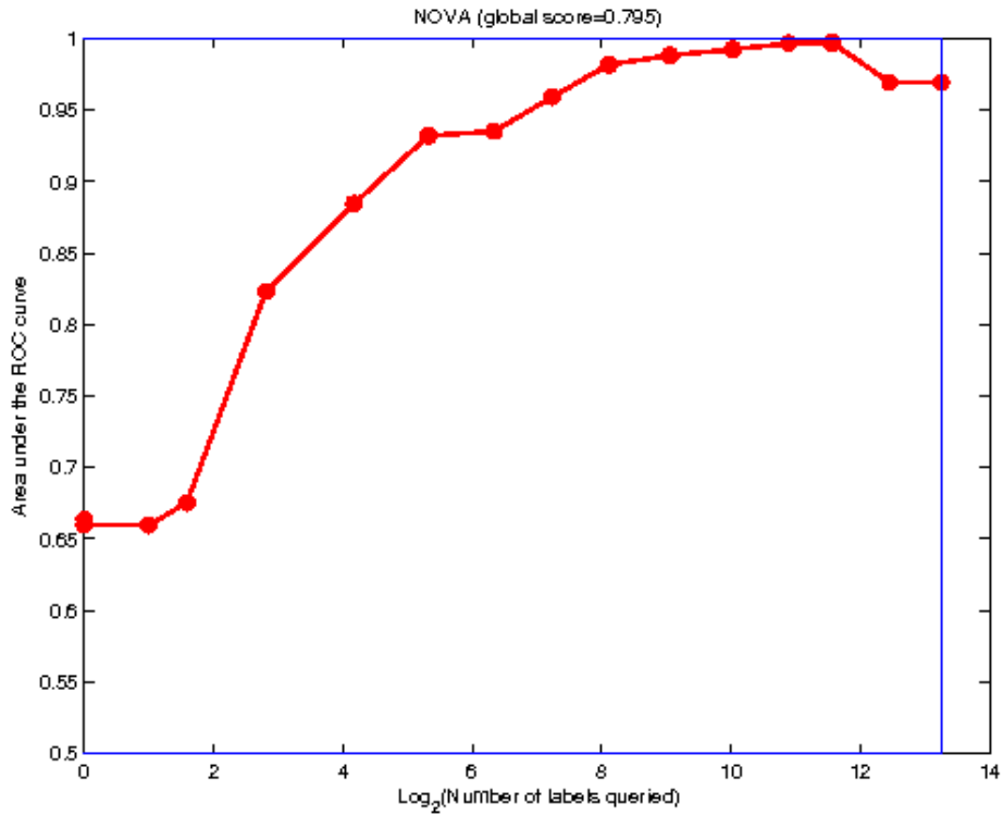
Reference results on NOVA by Gideon Dror.
