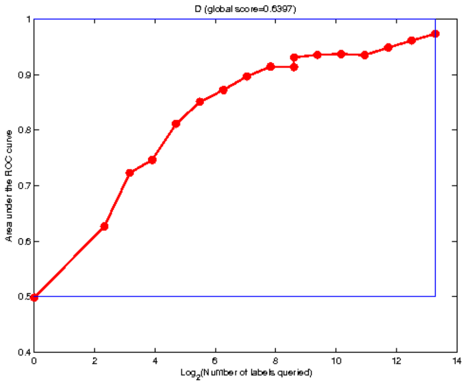
Results on dataset D by Ideal Analytics, Intel.
