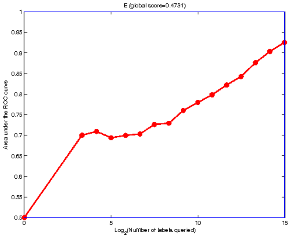
Results of IdealAnalytics, Intel, on dataset E
