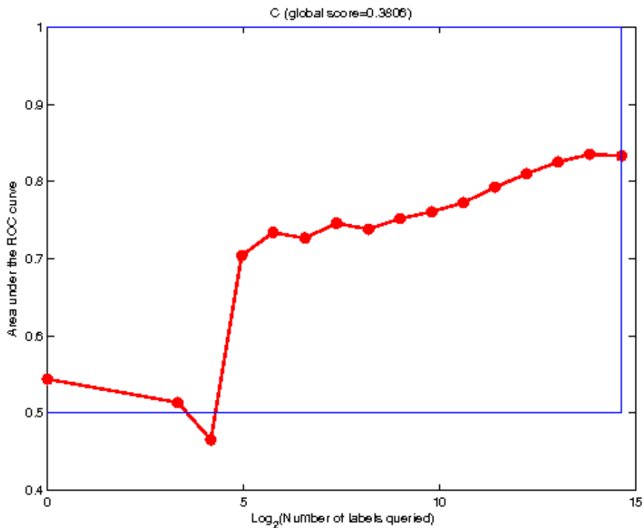
Results on the C dataset by Ideal Analytics, Intel.
