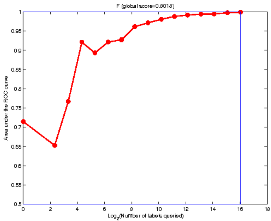
Results by Ideal Analytics, Intel, on the F dataset.
