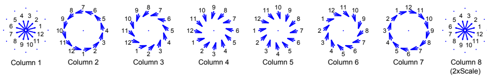
Figure 2: The construction of our 12 \times 8 \mathbf{P} -matrix descriptor. The arrangement is the same as in [1], but we base the descriptor on the 4S-DTCWT. The small numbers (and the orientations of the arrows) denote the subband selected at each sampling location. Each column is composed of a set of rotationally symmetric samples. The figure is taken from [1].
