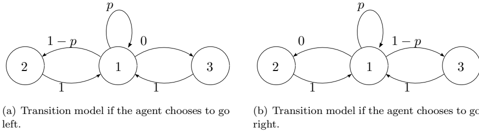
Figure 1: State transitions for Example 3.1. Taking the left action in state 1 leads to state 2 with probability 1-p . There is a small probability p of staying in state 1, regardless of the action taken; thus making the MDP aperiodic. From state 2 or 3, the agent moves to state 1 deterministically.
