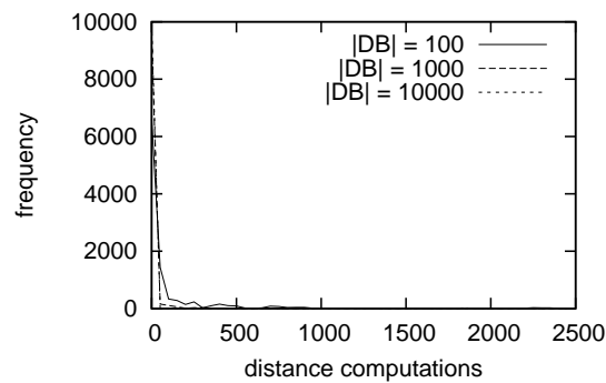
Histogram of distance computation caused by an insertion (dim = 10)
