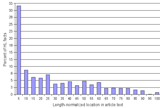
Figure 2: Positions of sentences from which high-lights (HLs) were generated.
