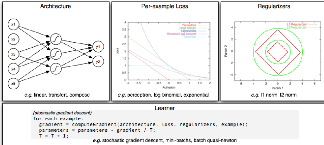
Figure 1: This figure illustrates the framework of energy-based models. Top: the three components that define the learning energy. Bottom: the learner component that performs energy minimization.
