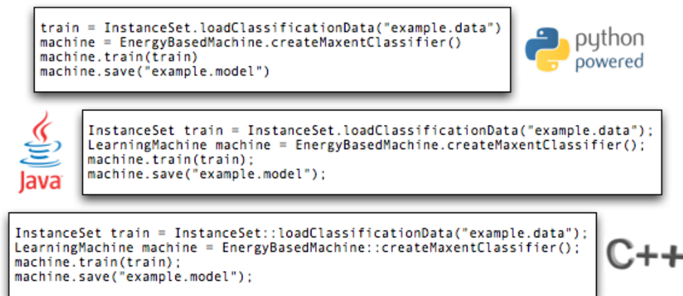
Figure 2: This figure shows the same program in three languages (Python, Java and C++). The program loads a classification data set, trains a maximum entropy classifier and saves the resulting model in a file called “example.model”.
