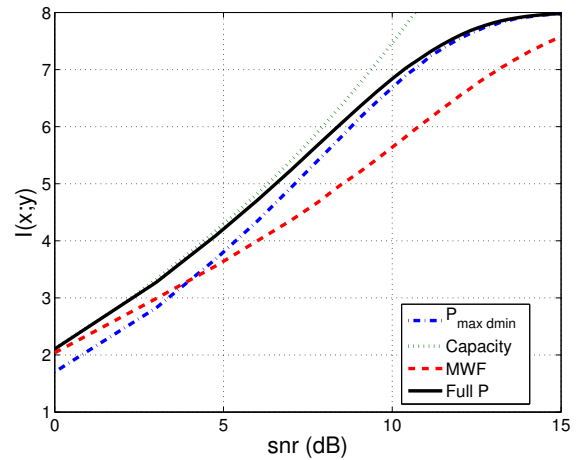
Fig. 3. Information transmission rates for the 4 \times 4 matrix in (16).
