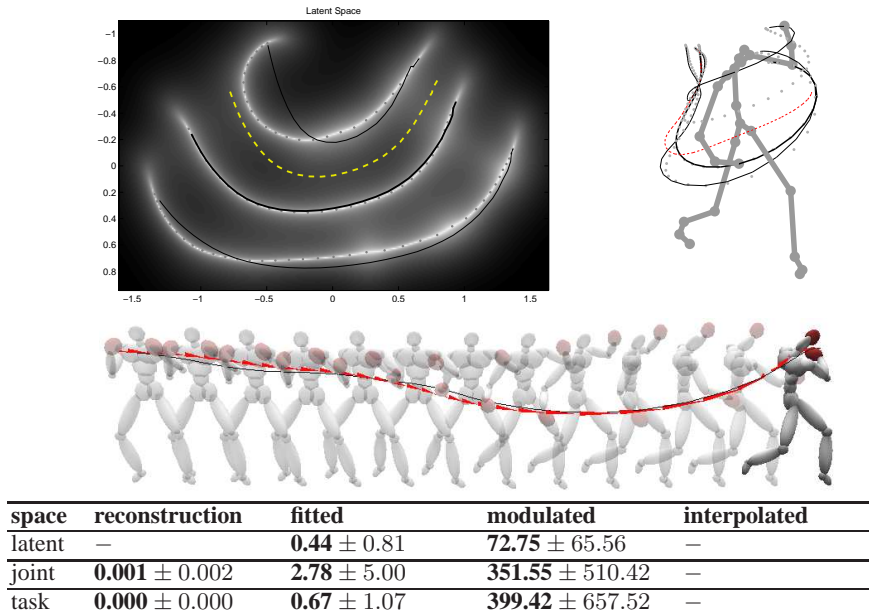
Fig. 5. Fitted (bold), modulated (thin) and interpolated (dashed) discrete Control Policies for the human punching motion in latent and end effector space. MIDDLE: Very low punch with path of right hand for original punch (red triangles) and result from CP modulation (solid line). BOTTOM: Errors for human movements (nMSE \times 10^{-3} together with its standard deviation).
