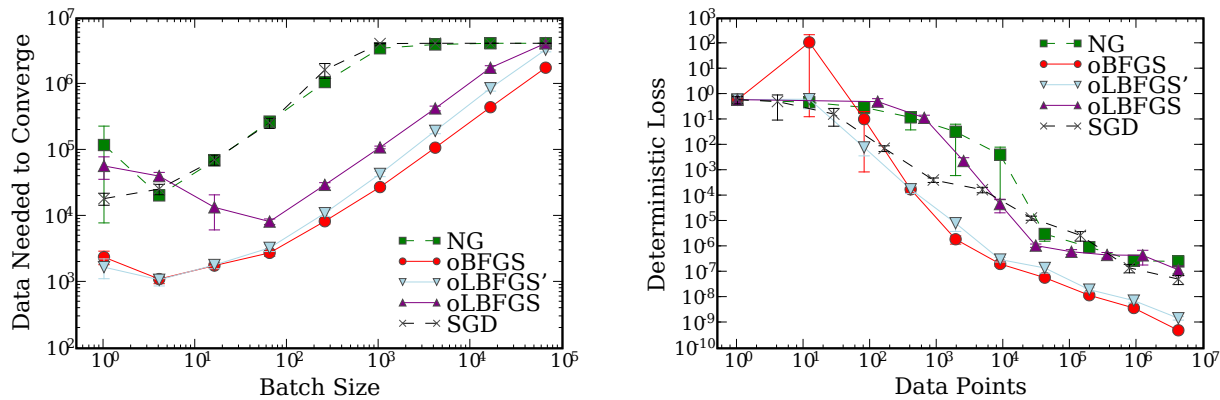
Figure 2: Average performance (with standard errors) of stochastic gradient methods on the non-realizable quadratic (16) with \sigma = 10^{-2} over 10 matched random replications. Left: number of data points needed to converge to f(\theta) < 10^{-5} , up to a limit of 2^{22} , vs. batch size b . Right: deterministic loss f(\theta) vs. number of data points seen, at the optimal batch size for each algorithm. All methods used (7) with \eta_0 and \tau tuned for fastest convergence at small batch sizes: \eta_0 = b/(b+2), \tau = 10^4 (SGD); \eta_0 = 0.04, \tau = 20 (NG); \eta_0 = b/(b+2), \tau = 20 (oBFGS); \eta_0 = 0.1 \cdot b/(b+2), \tau = 2 \cdot 10^4 (oLBFGS); \eta_0 = b/(b+2), \tau = 10 (oLBFGS'); \lambda, c, m as in Figure 1.
