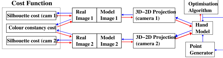
Fig. 1. Flow diagram showing the components making the tracking system
