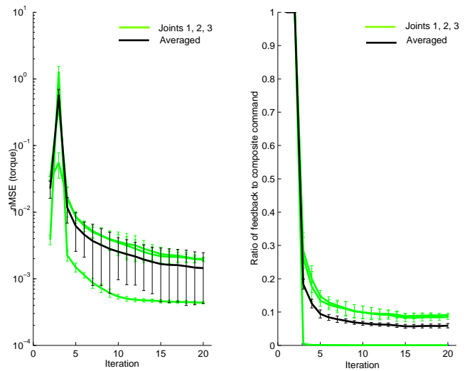
Fig. 3. Learning performance of LWPR over 6 different loads and 20 iterations. Left: normalized MSE on the test data. Right: average contribution of the error-correcting feedback PD control.
