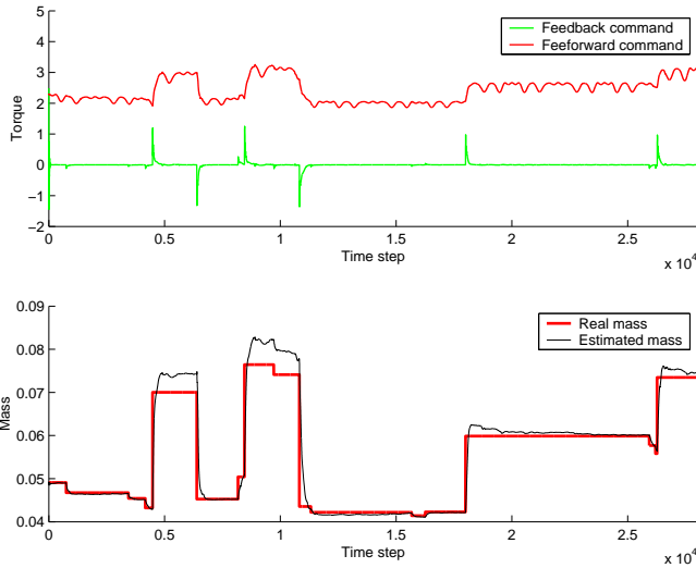
Fig. 5. Load estimation and control of non-stationary loads. Top: contribution of feedforward and feedback command. Bottom: real and estimated mass.
