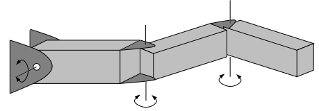
Fig. 2. Simulated 3DOF arm
