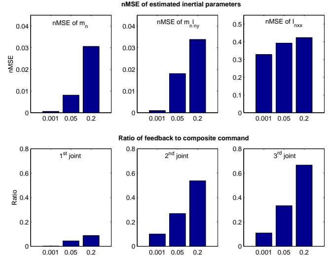
Fig. 6. Effect of imperfect dynamic models
