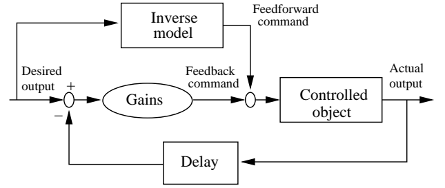
Fig. 1. The composite controller
