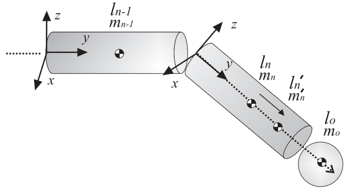
Fig. 4. In our experiments, both the center of mass of the last link l_n and the load l_o are constrained to lie on the y axis of the last link's reference frame, so that the center of mass of their union \hat{l}_n also lies on the y axis.
