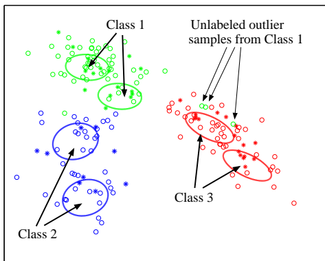
Fig. 1. SDCA-GM result on Wine data (178 points from 3 classes). A two-dimensional subspace was sought for originally 13-dimensional data. The labels of 20% of the points (denoted by ‘*’) were known in the training. The labels of the rest of the points (denoted by ‘o’) were not revealed during training. The points are shown in the found two-dimensional space. Ellipses show the location and shape of the Gaussian components used to model each class.
