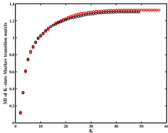
Fig. 3. The mutual-information (MI) score of the clustered Markov process as a function of the number of clusters. The black circles indicate MI values based on equal-time division features. The red circles indicate MI values as a function of equal-distance division features.
