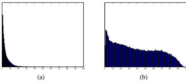
Fig. 5. (a) A squared differences histogram between segments within one cluster of Markov states (b) A squared differences histogram between segments from different clusters of states.
