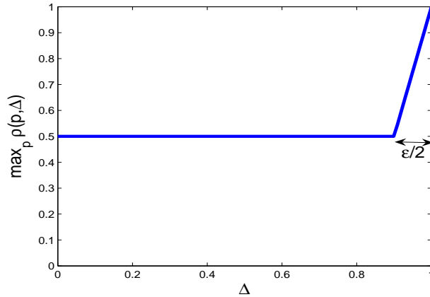
Figure 2: The function \Delta \mapsto \max_p \rho(\mathbf{p}, \Delta) for Example 2.1.
