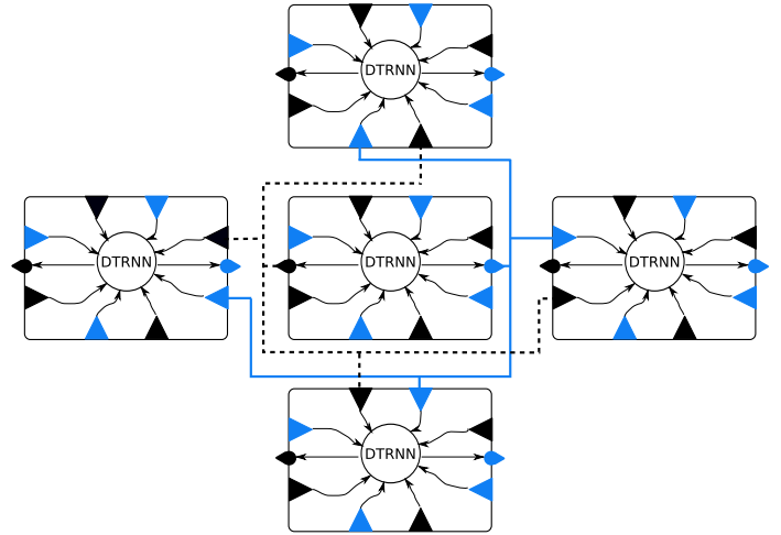
Figure 1: Schematic view of the connections between cells in the case of 2 chemicals
