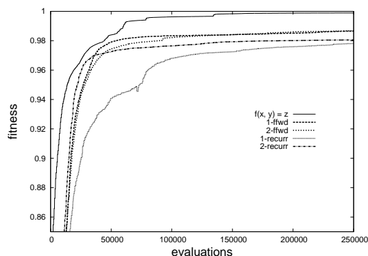
Figure 6: Evolution of average of best fitness for the 3-bands problem. The lowest curve is that of the 1-recurr model , and the 3 indistinguishable curves above the other 2 are those of the other 3 artificial embryogeny models.
