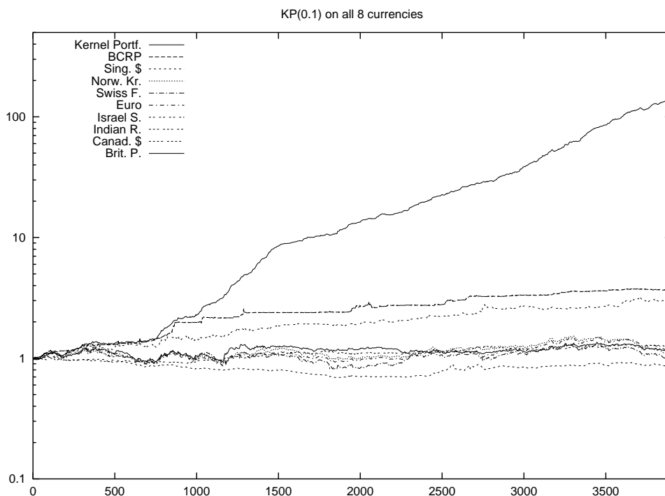
Figure 1: Wealth achieved along N = 3900 daily periods by investing one US$ in several currencies, and by using the kernel-based strategy computed with d = 8 currencies, like in column five of Table 3. Horizontal axis is time period number, vertical is the wealth achieved, in logarithmic scale.
