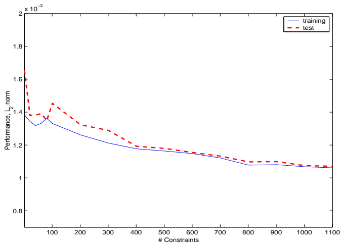
Figure 3: The average training (blue unbroken) and test (red dashed) L_2 error as a function of the number of constraints (size of the sample m_f ) – sample size m_x = 50
