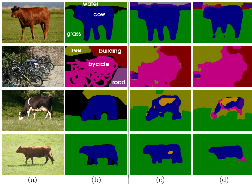
Fig. 6: Class segmentation results. (a) Original photographs. (b) Ground-truth class labels. (c) Output class maps obtained with KL divergence. (d) Output class maps obtained with L2 distance. In most cases L2 gives less accurate segmentation. In all cases our single-histogram class models were used, together with 5 \times 5 patch features, V = 8000 and K-means clustering.
