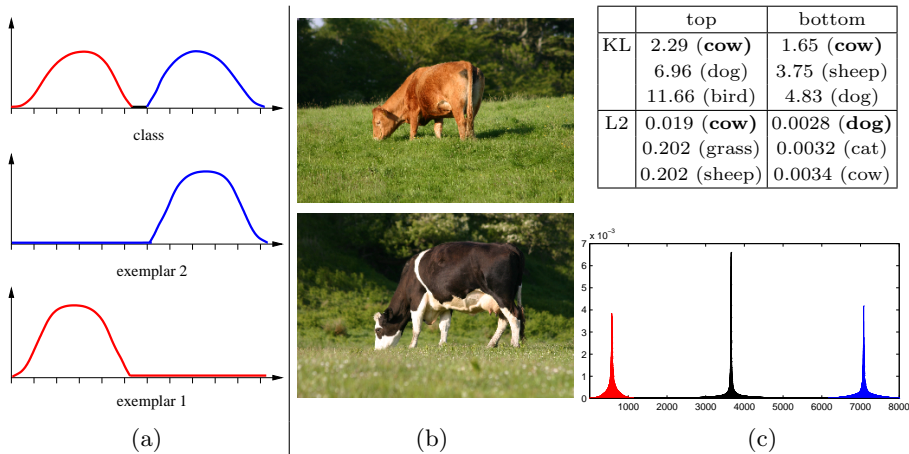
Fig. 5: Advantages of KL. Different instances of cows induce different proportions of visual words. A unified “cow” model histogram (c) will contain different “modes” for the different visual aspects and species of the instances. (a) provides a schematic visualisation. In (c) the mode corresponding to the top cow in (b) is shown in red (left), and for the bottom cow in blue (right). The remaining visual words of the cow -model are shown in black in the middle. Note that a simple sorting of the visual words has been employed to bring out the different modes. The table shows the distances of the cow exemplars in (b) to the class models (showing the nearest class in bold). KL divergence ignores zero bins in the query histograms and is thus better suited for this scenario (note the wrong classification with L2 for the bottom cow).
