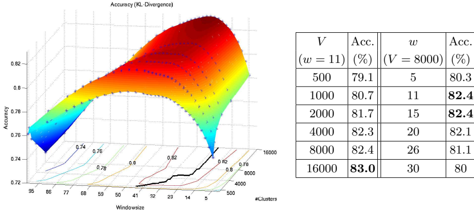
Fig. 4: Accuracy analysis on the 6-class set. Pixel-wise classification performance as a function of the size w of the sliding window and the size V of the visual vocabulary. The features are 27-dimensional 3 \times 3 CIE-LAB patches. The vocabulary is learnt by K-means clustering run for 500 iterations. KL divergence is used for histogram comparisons.
