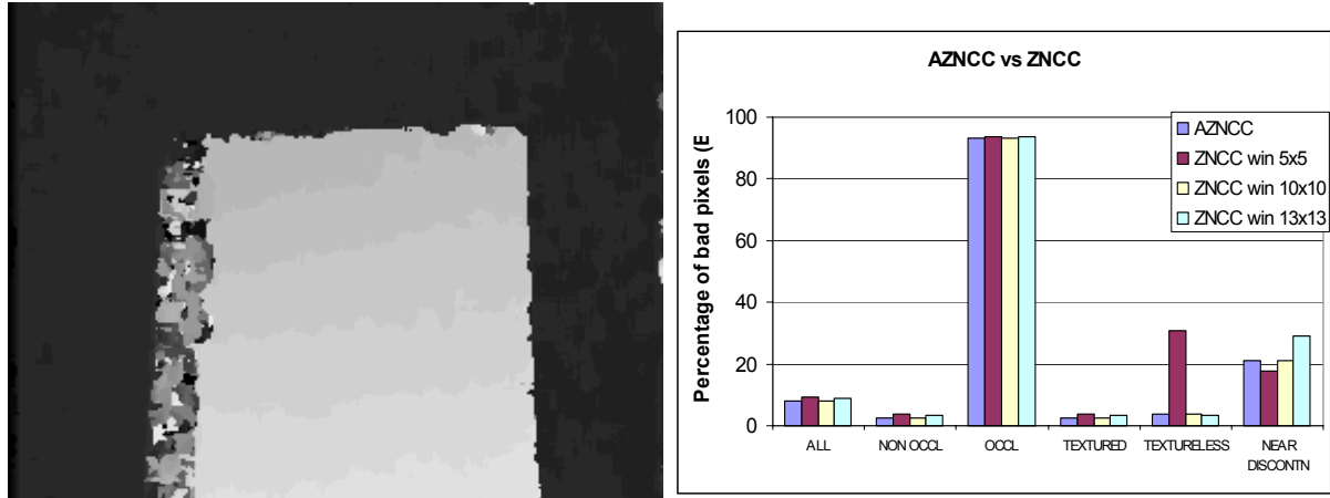
Figure 9 Disparity map and plots of performances obtained by AZNCC and local algorithms implementing the matching cost ZNCC and 5X5, 10X10 and 13X13 aggregation windows.
