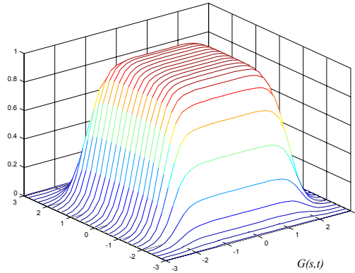
Figure 2 - Function G(s,t) , component of the activation function obtained as difference of two sigmoid functions
