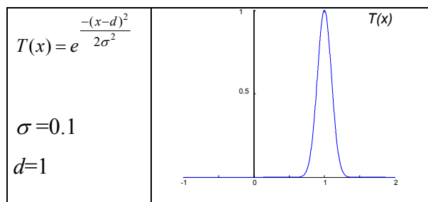
Figure 3 - Neuron transfer function T(x) ; d and \sigma centre and standard deviation respectively; the function is exemplified for d=1 and \sigma=0.1
