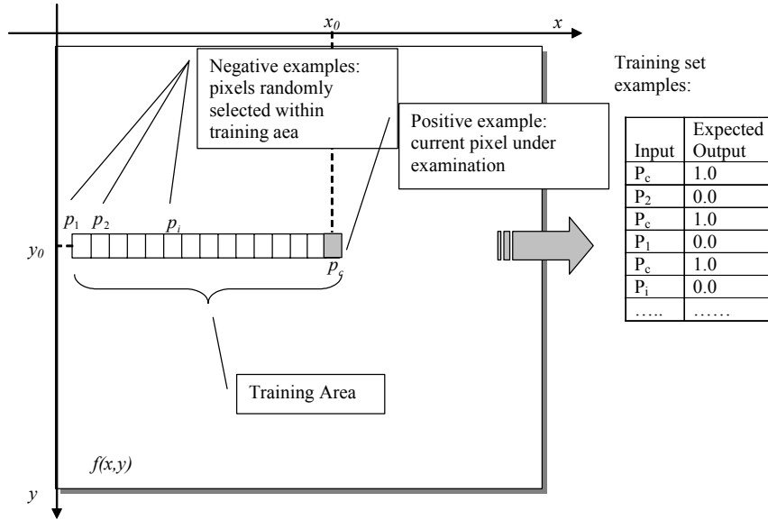
Figure 4 - Exemplification of training set construction
