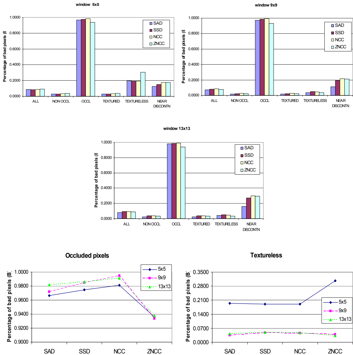
Figure 6- Performances of different matching costs aggregated with 5X5, 9X9 and 13X13 window and applied on MAP image
