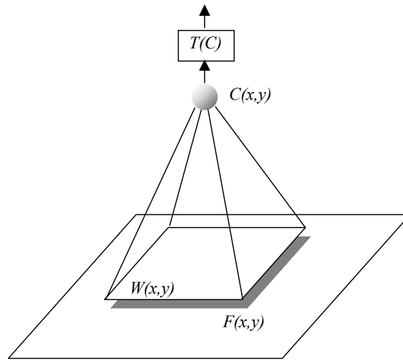
Figure 1 – Neural Representation of Correlation Measure
