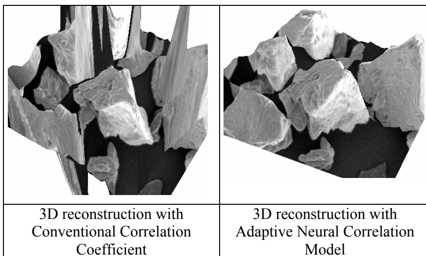
Figure13 – a-reference and target images of specific preparations of inorganic crystals (NaCl). b- surface reconstructions obtained with conventional Correlation Coefficient and Adaptive Neural Correlation Model
