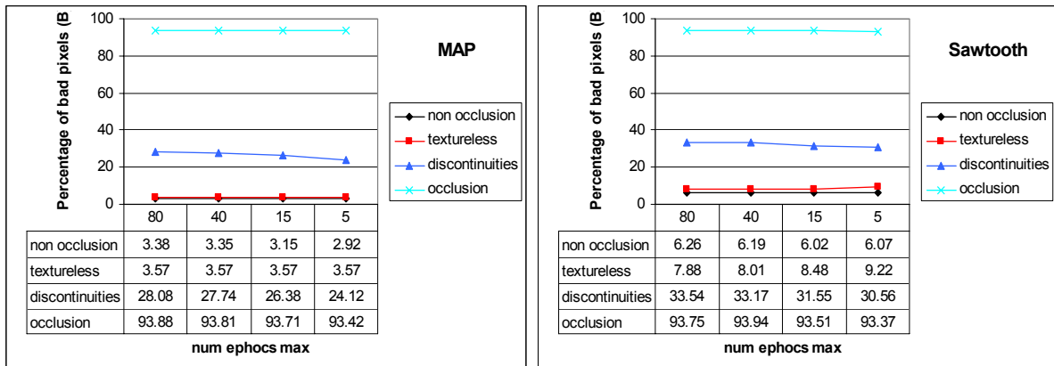
Figure 7 Plots of the performances of AZNCC as function of maximum number of epochs
