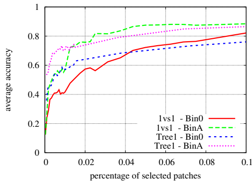
Figure 7: Automatic binarization increase the performance of lvs1 and tree
