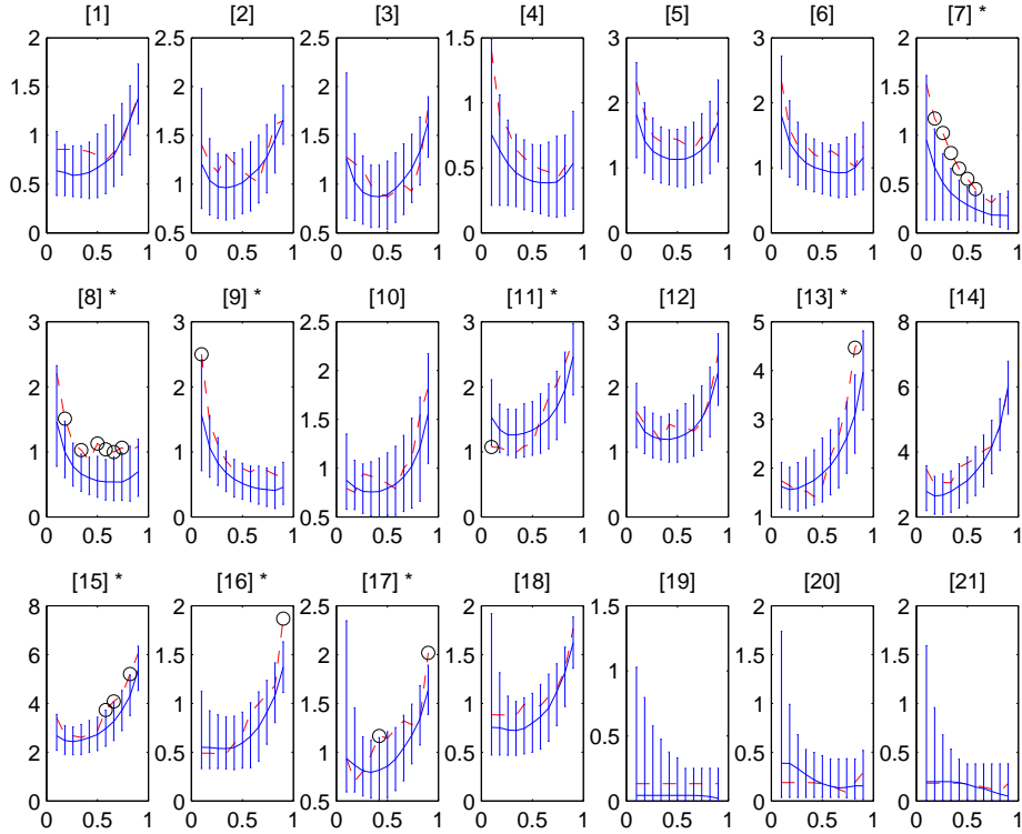
Fig. 2. The EPC curve range (due to 1000 samples of random identity match) at 95% of confidence versus the EPC curve of true identity match, for each of the 21 experiments, using the mean operator as the fusion classifier. They are labeled accordingly from 1 to 21 corresponding to the experiment numbers in Table 2. A * sign is marked for the experiments whose one or more HTERs of true identity match fall outside the confidence range. For these points, circles are plotted on the corresponding EPC curve.
