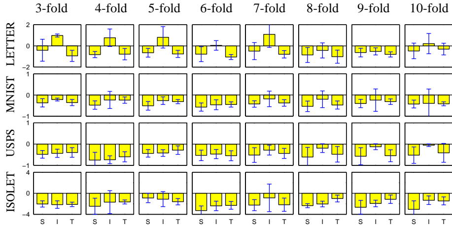
Figure 2: Comparison of the three data-driven averaging conversions with the data-independent conversion, for different datasets (Y-axis) and different training-set sizes (X-axis). Each bar shows the difference between a data-driven conversion ( suffix (S), interval (I) or tree-based (T)) and the data-independent conversion.
