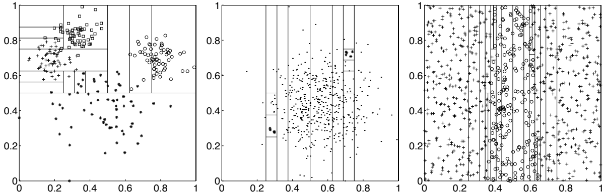
Figure 4: Left: Solution in a four class setting. Middle: Solution obtained for an extremely unbalanced problem. The small class of interest (8 points) is concentrated in two regions. Right: Solution obtained for an anisotropic situation where the true boundary separating the classes is defined by two straight lines with small, but non-zero, inverse slope.
