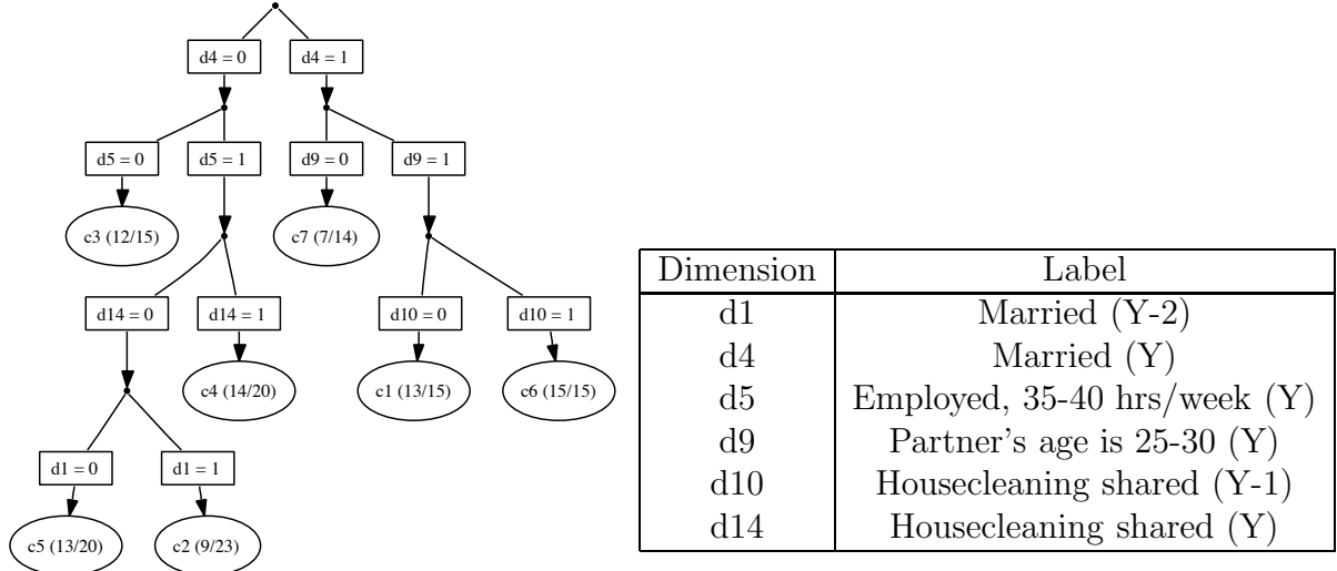
Figure 6: The derived trees for the german fertility dataset (122 examples, 7 classes, 17 binary dimensions). In each leaf the numbers x/z indicate the number of examples in the majority class ( x ) and the total number of examples in the leaf ( z ). Each feature corresponds to an answer to a questionnaire for a given year prior to the conception of the child. In the feature description, Y is the year of conception of the child (birth minus 10 months).
