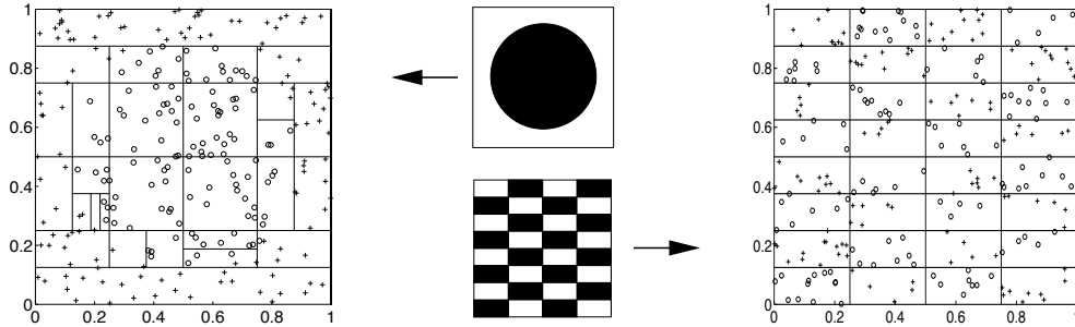
Figure 3: The two artificial classification problems and an instance of the output of the ODT algorithm: (left) 'circle' example, (right) 'checkerboard' setup. In the middle we show a cameo of the true class separations.
