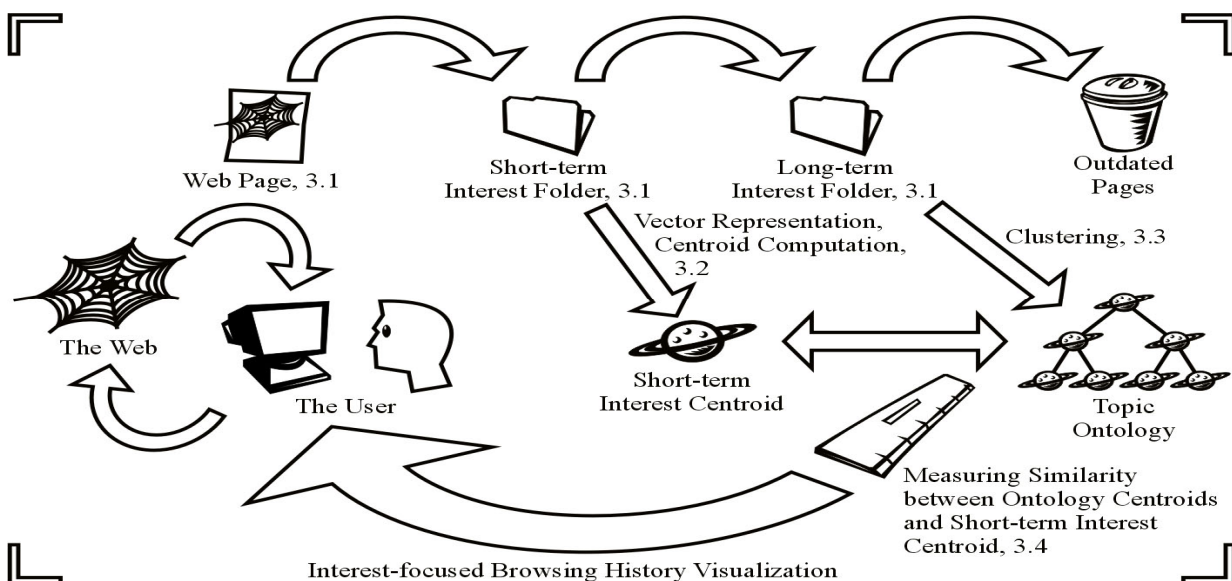
Figure 1. The Interest-focused Browsing History Architecture. The process is described throughout Section 3. The corresponding subsections are noted in the figure (3.1, 3.2, 3.3, 3.4)
