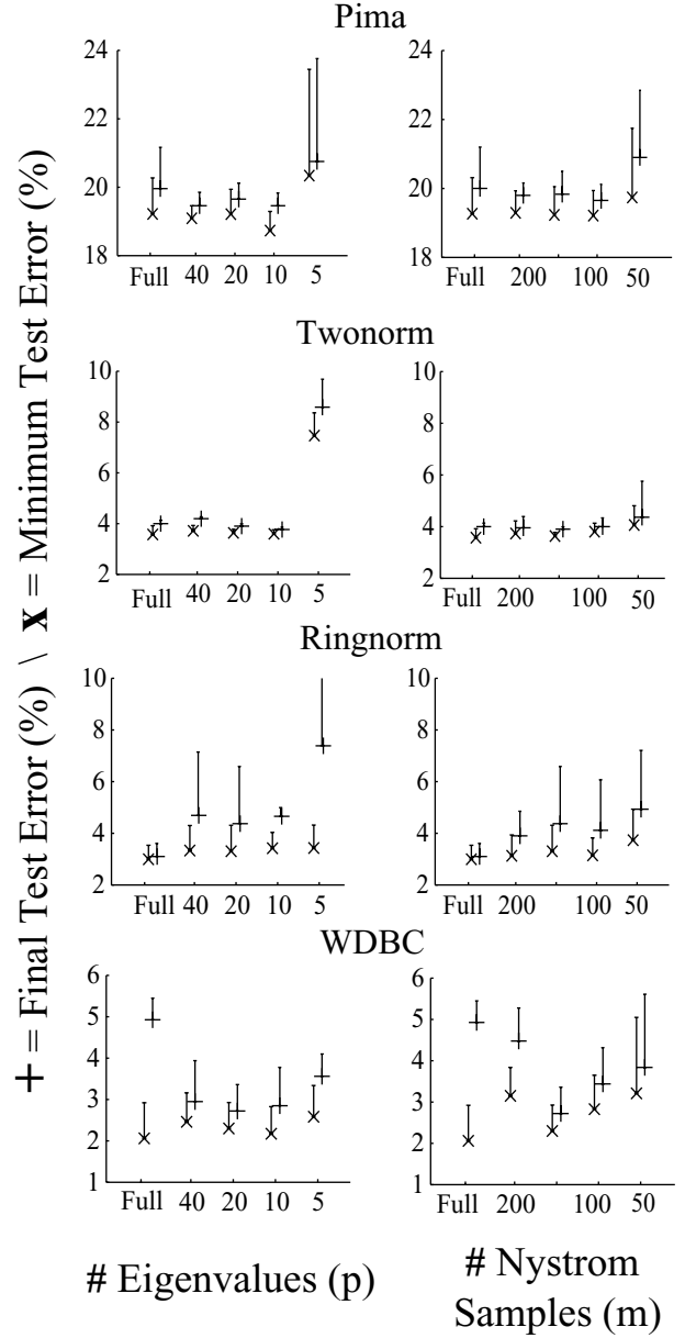
Fig. 1. Comparison of test errors (minimum and final) achieved for the Bayesian evidence gradient ascent Nystrom HMC hyperparameter tuning with varying numbers of eigenvalues, p (left column), and samples in the Nystrom approximation, m (right column). For the left column m = 150 , and for the right column p = 20 . For reference, results are also shown for the standard HMC with p = m = n [9] ('Full'). Markers show averages over 25 trials. One-standard deviation error bars are shown 'pessimistically', i.e. only upwards from the mean, because the error distributions are highly skewed in this direction [9].
