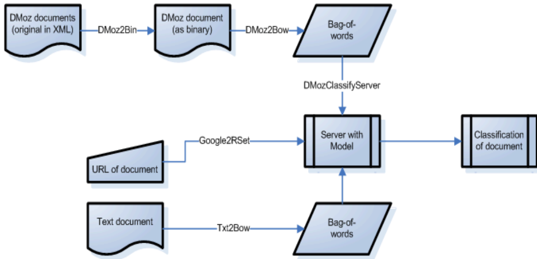
Figure 1. Architecture of the system for extracting human expertise from DMOz topic ontology.
