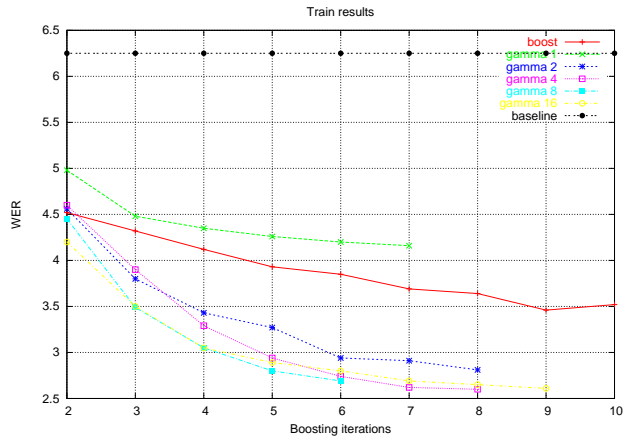
Fig. 1. Training word error rates for various values of gamma, compared with a number a baseline system and the previous boosting approach.
