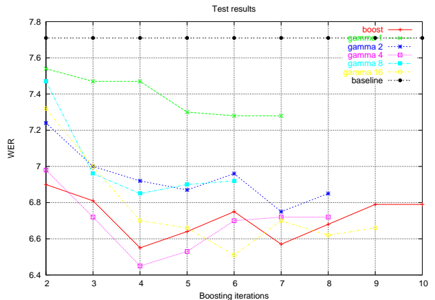
Fig. 2. Test word error rates for various values of gamma, compared with a number a baseline system and the previous boosting approach.
