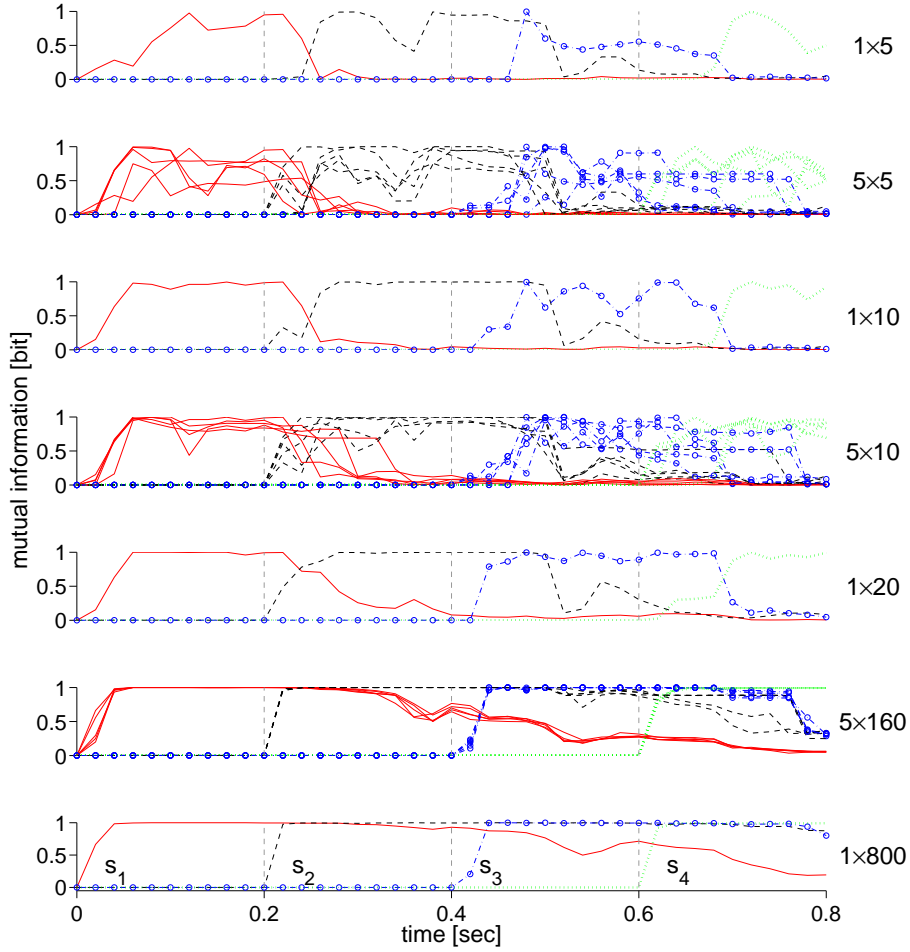
Figure 4: Information in subset of neurons. Shown are lower bounds for mutual information MI(s_i, h(R)) obtained with a linear classifier h operating on d components of the circuit state \mathbf{r}(t) . The numbers a \times d to the right of each panel specify the number of components d used by the linear classifier and for how many different choices a of such subsets of size d the results are plotted in that panel.
