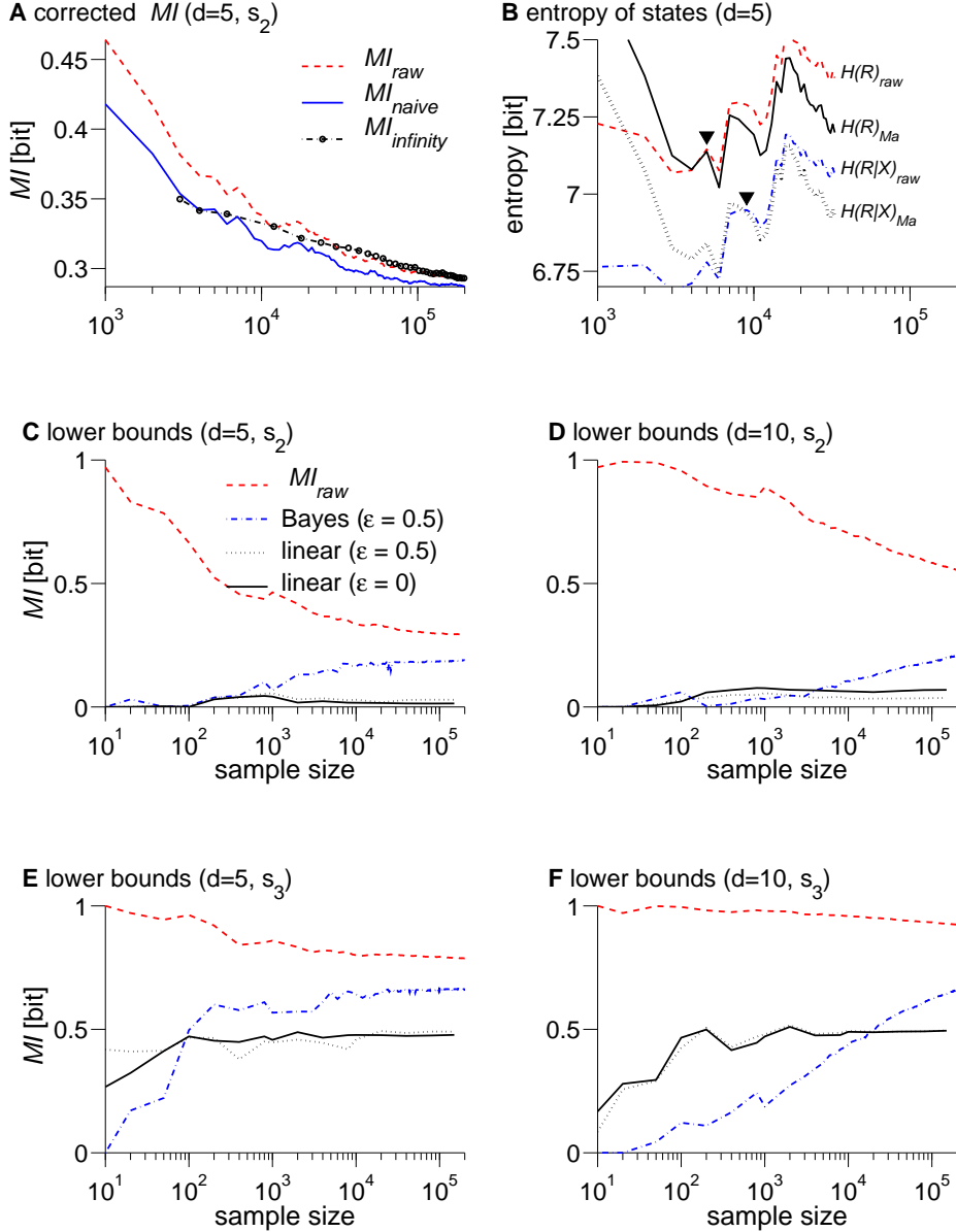
Figure 3: Estimated mutual information depends on sample size. In all panels d denotes the number of components of the circuit state \mathbf{r}(t) at time t = 660 ms (or equivalently the number of neurons considered). A Dependence of the “raw” estimate MI_{raw} and two corrected estimates MI_{naive} and MI_{infinity} of the mutual information MI(s_2, R) (see text). B Estimates of the entropies H(R) and H(R|X) . The “raw” estimates are compared with the corresponding Ma-bounds (see text). The filled triangle marks the sample size from which on the Ma-bound is below the raw estimate. C Lower bounds MI(s_2, h(R)) for the mutual information obtained via classifiers h which are trained to predict the actual value of s_2 given the circuit state \mathbf{r}(t) . Results are shown for a) an empirical Bayes classifier (discretization \epsilon = 0.5 , see footnote 3 and 5), b) a linear classifier trained on the discrete ( \epsilon = 0.5 ) data and c) for a linear classifier trained on the analog data ( \epsilon = 0 ). In the case of the Bayes classifier MI(s_2, h(R)) was estimated by employing a leave-one-out procedure (which is computationally efficient for a Bayes classifier), whereas for the linear classifiers a test set of size 5 \cdot 10^4 was used (hence no results beyond a sample size of 1.5 \cdot 10^5 ). D Same as C but for d = 10 . E Same as C but for MI(s_3, h(R)) . F Same as E but for d = 10 .
