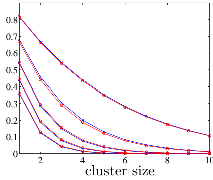
Figure 8. Probability of absence of a cluster vs. cluster size for subsampling with ( \circ ) and without ( \times ) replacement for a training sample size of n = 50 . From top to bottom, subsample size is n' = 10, 20, 30, 40, 50 with replacement, and 9, 16, 23, 28, 32 \simeq n(1 - \exp(-n'/n)) without replacement.
